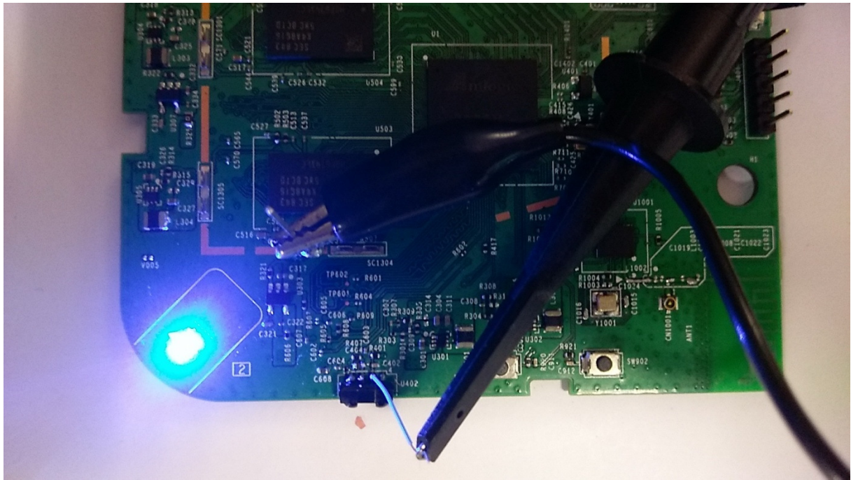
Figure 3: Measurement point of IR Receiver output of T99X171T00
